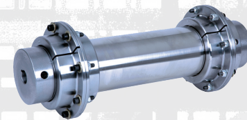
Double-Ended Spacer Couplings Shown with high-speed split cover
